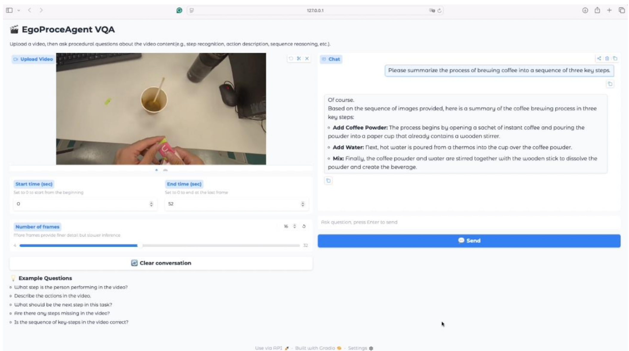
(d) Visualization interface example: Identifying the key step sequence of making coffee in the video.
